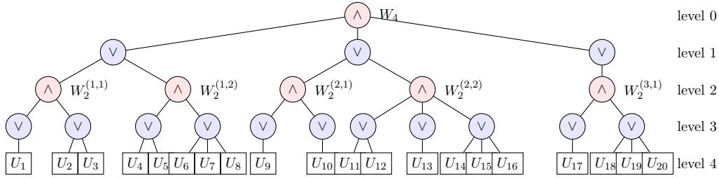
FIGURE 1.1. An example of a minimax tree, with 4 levels. Here all non-leaf nodes have 1, 2 or 3 children.
