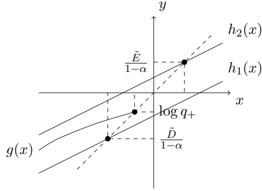
FIGURE 4.1. h_1(x), g(x), h_2(x) together with their (stable) fixed points \frac{\tilde{D}}{1-\alpha}, \log q_+, \frac{\tilde{E}}{1-\alpha} respectively. For x \leq \log q_+ , h_1(x) \leq g(x) \leq h_2(x) . The dashed line represents the identity function.
