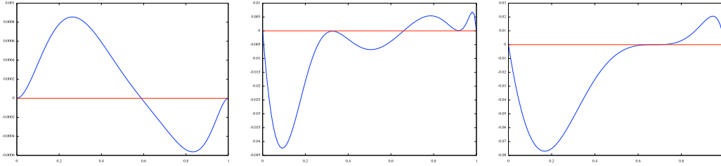
FIGURE 2.2. The function f(x) - x for x \in [0, 1] in three further cases: (a) p_1 = 0.5 , p_2 = 0.25 , p_4 = 0.25 ; (b) p_2 = 0.783 , p_{30} = 0.217 , and (c) p_2 = 0.705 and p_{12} = 0.295 .
